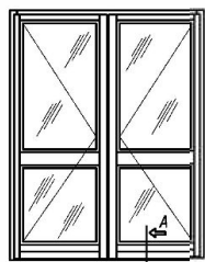
VERTICAL SECTION
